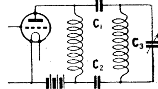
Fig. 9.—A similar method modified so that the H.T. battery is removed from the main oscillatory circuit.
