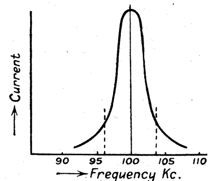
Fig. 4.—This curve has a flatter top, but the cut-off is too sharp for good quality.
